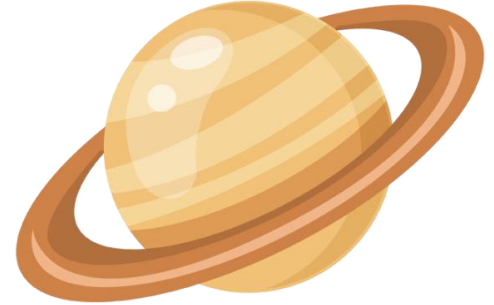
Saturn
